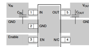
Figure 7-7. DBV Package (SOT-23) Typical Layout
